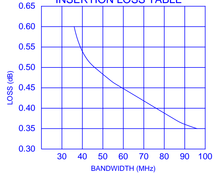
INSERTION LOSS TABLE
